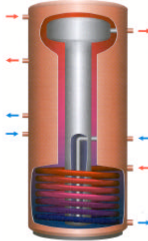
Tank in Tank
