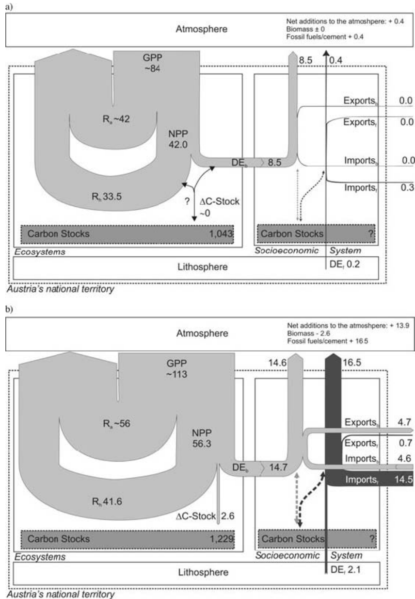
Figure 4 Average annual carbon flows in Austria in the periods 1830–1880 (panel A) and 1986–2000 (panel B). Arrow sizes are proportional to the magnitude of the carbon flows. Flows are reported as MtC/yr, and stocks are reported as MtC. Import/Export f = foreign trade with fossil fuel products; Import/Export b = foreign trade with biomass products. Dashed arrows indicate that the flows were not considered. GPP and R_a calculations are provided only for illustrative purposes. The very thin vertical arrow in Figure 4a represents the socioeconomic carbon flow associated with fossil fuel use. GPP = gross primary production; R_a = plant respiration; R_h = heterotrophic respiration; NPP = net primary production; \Delta C = stock = net change of carbon stocks in ecosystems; DE = domestic extraction.
