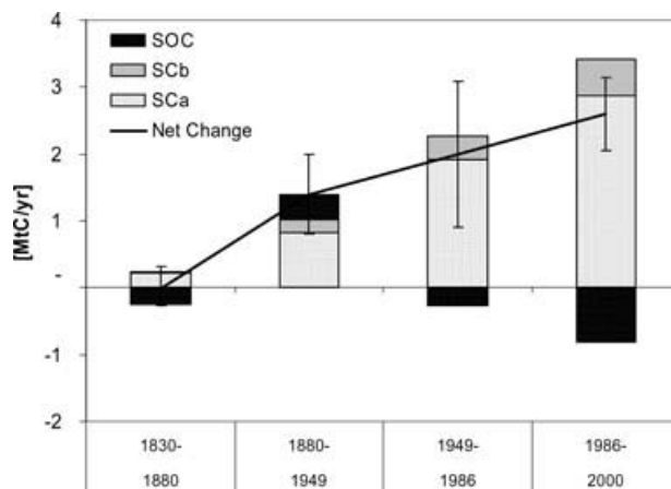
Figure 3 Average annual net carbon flows between the atmosphere and different vegetation compartments in four periods from 1830 to 2000. Positive values indicate carbon sinks (flows from the atmosphere); negative values indicate carbon sources (flows to the atmosphere).
