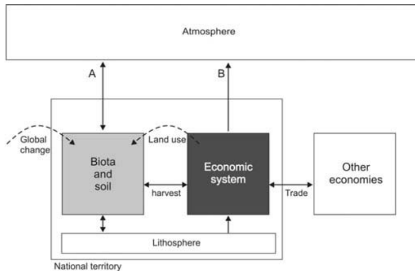
Figure 1. Systematics of the national carbon flows quantified in the study. Solid-line arrows indicate carbon flows. Dashed arrows indicate impacts. A: carbon uptake and release of ecosystems; B: carbon flows resulting from socioeconomic processes.
